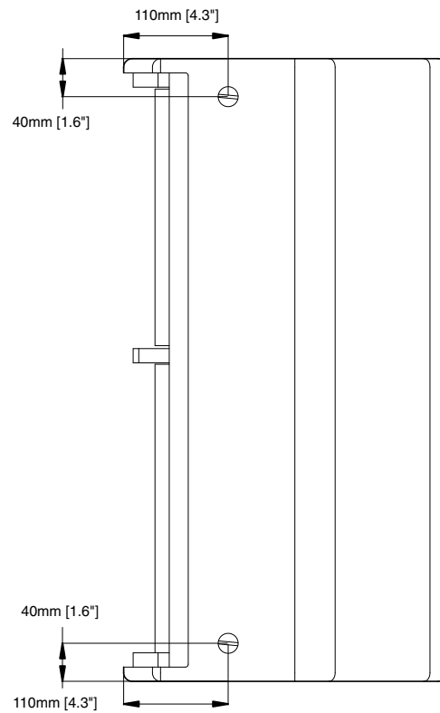
SIDE
