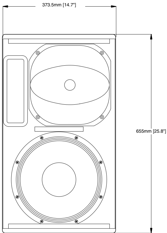
FRONT
